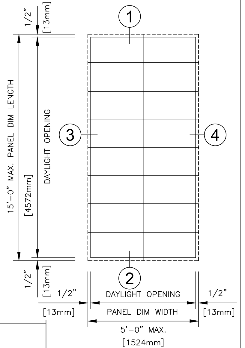
PANEL ELEVATION
