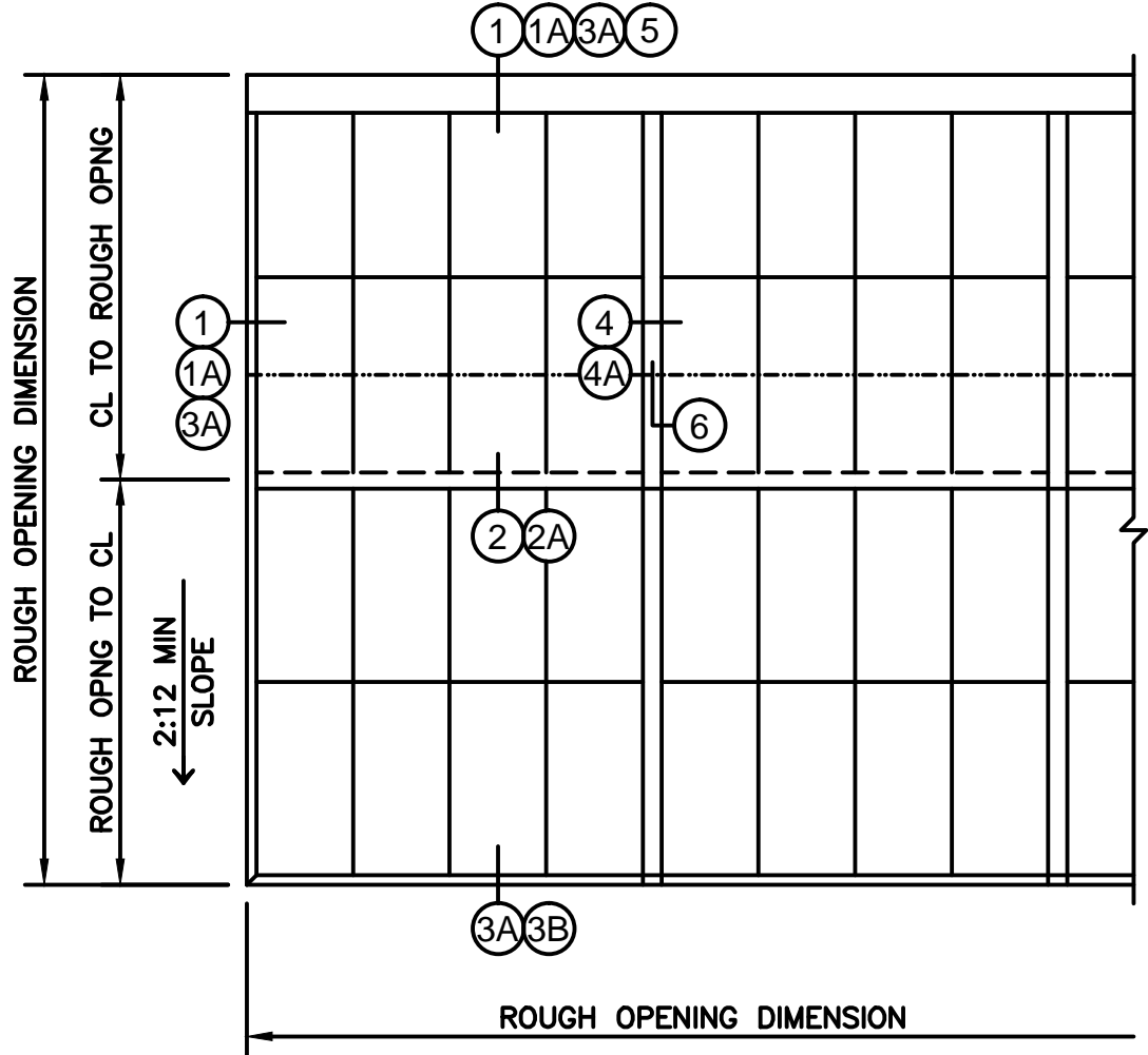
ROOF PLAN
